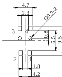
P.C.B. Layout for SPFSC
