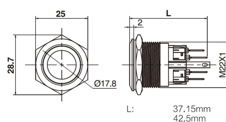
RJS103-22L(A)-F-R~67J
