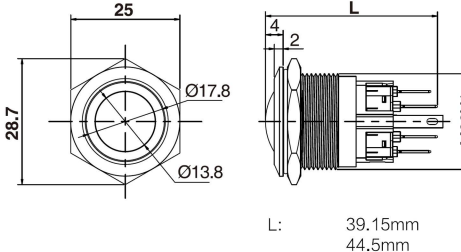
RJS103-22L(A)-B-R~67J
