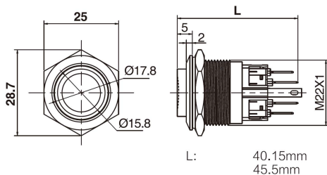
RJS103-22L(A)-H-R~67J
