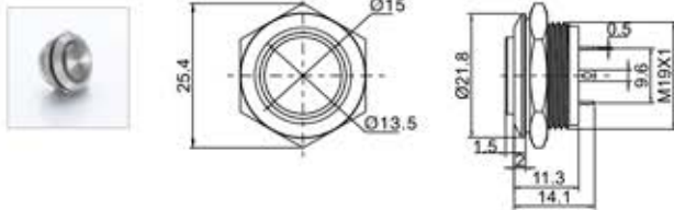
RJS1N1LP-19M-H-R~67J
