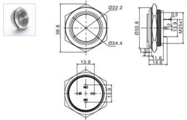
RJS1N1LP-30M-H-R~67J
