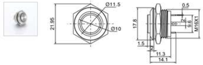
RJS1N1LP-16M-H-R~67J
