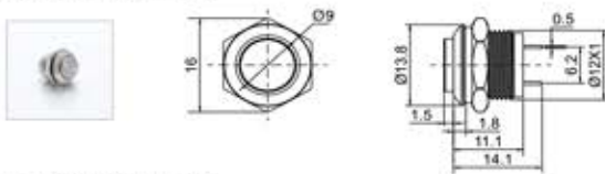
RJS1N1LP-19M-H~67J
