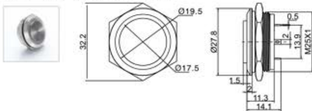
RJS1N1LP-25M-H-R~67J
