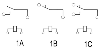
Wiring diagram(Bottom view)
