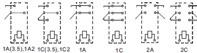
Wiring diagram (Bottom view)
