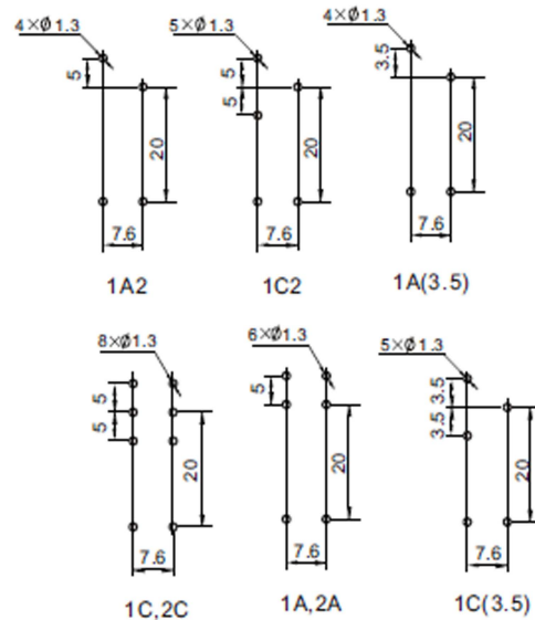
Mounting (Bottom view)
