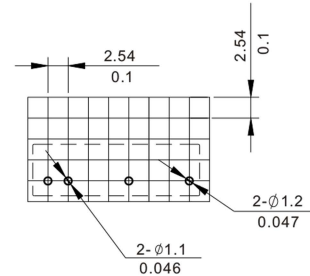
Mounting (Bottom view)
