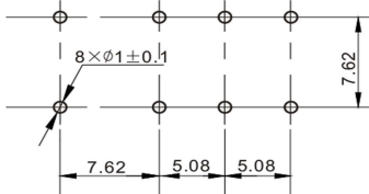
Mounting (Bottom view)
