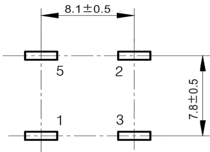
Mounting (Bottom view)
