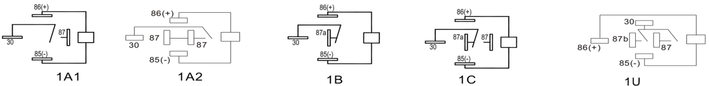
Wiring diagram (Bottom view)
