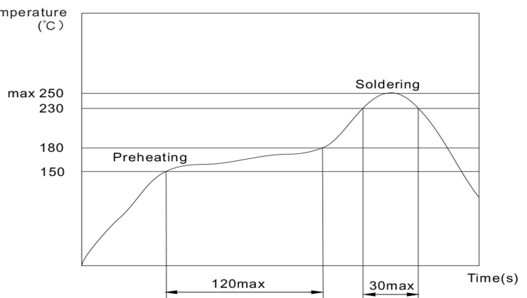
Reflow Soldering, Temperature on PCB Board
