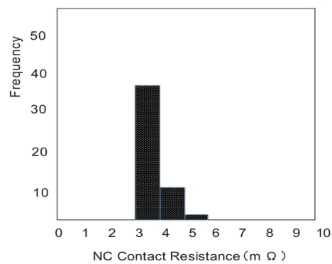
Sample : NG8N-1 DC12V 225Ω 50pcs
