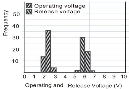
Sample: NG8N-1 DC12V 225Ω 50pcs
