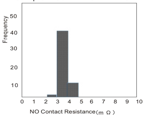
Sample: NG8N-1 DC12V 225Ω 50pcs
