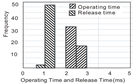
Sample: NG8N-1 12VDC 225Ω 50pcs Diode to absorb coil surge, without resistor
