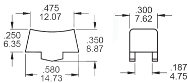
PANEL MOUNTING-R1
