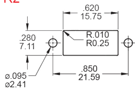
PANEL MOUNTING-R2
