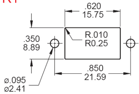
PANEL MOUNTING-R1
