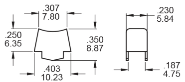
PANEL MOUNTING-R3
